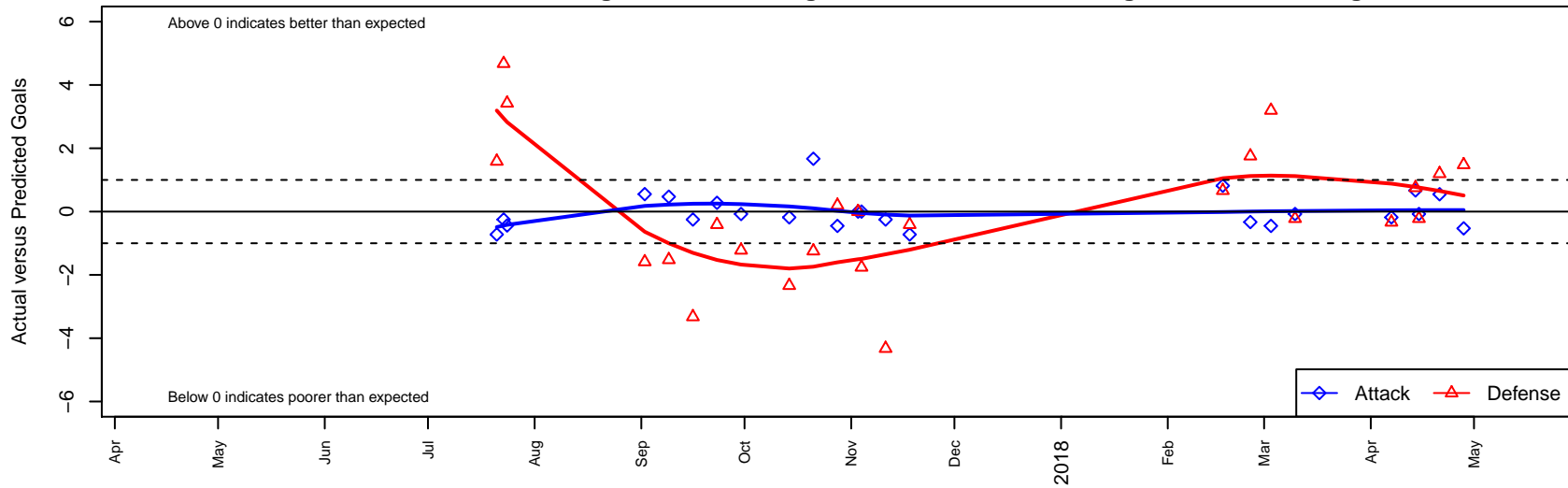
Snohomish United USSDA B05 Dots are actual minus expected GF (blue circles) and GA (red triangles). Blue line is smoothed change in attack strength. Red is smoothed change in defense strength.
